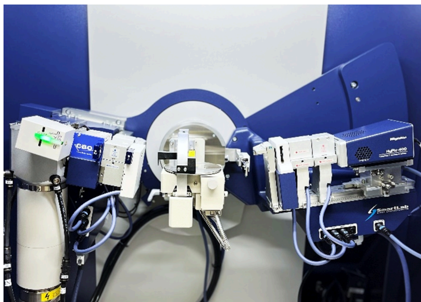
Figure 1: SmartLab SE with HyPix-400 detector and \chi\phi attachment
